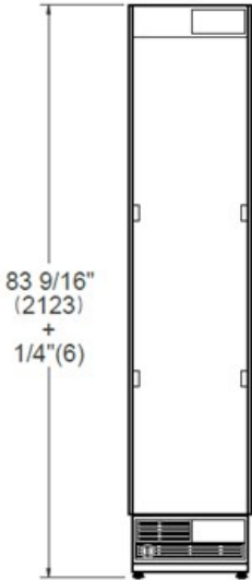
FRONT VIEW
